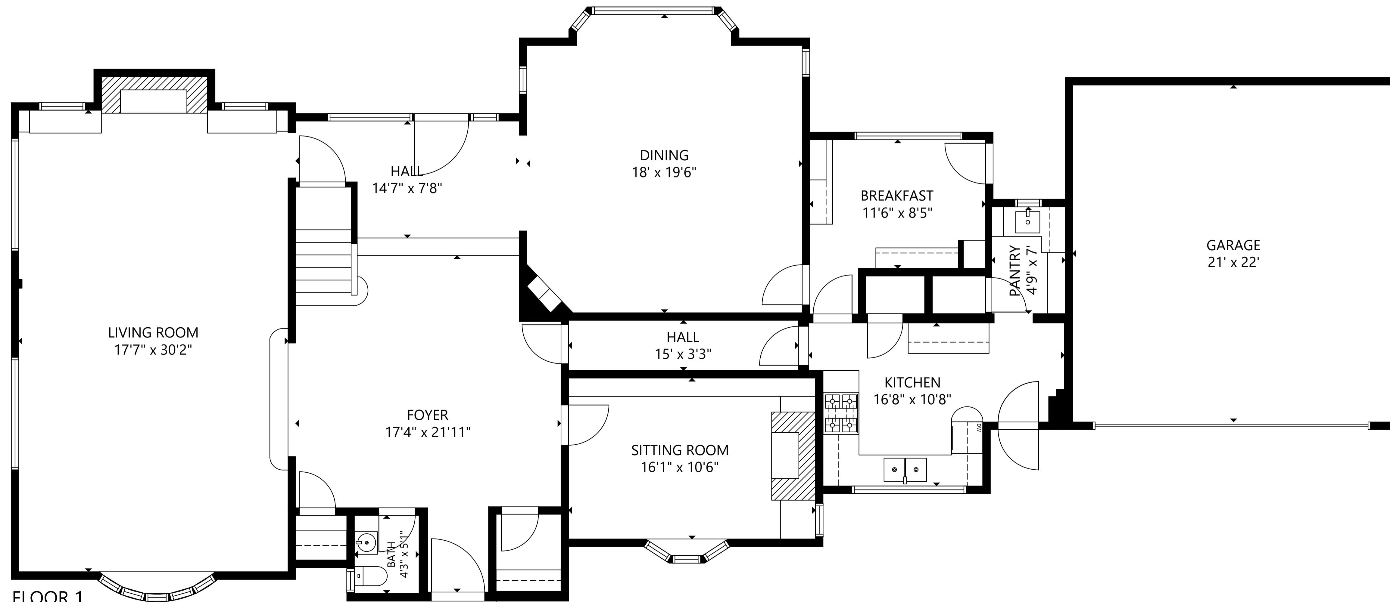
FLOOR 1
